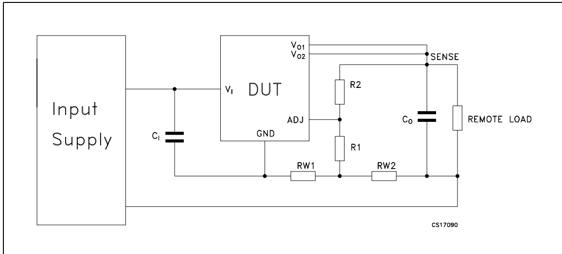
Figure 3. Application diagram for remote sensing operation
