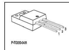
PG-TO220-3-31
