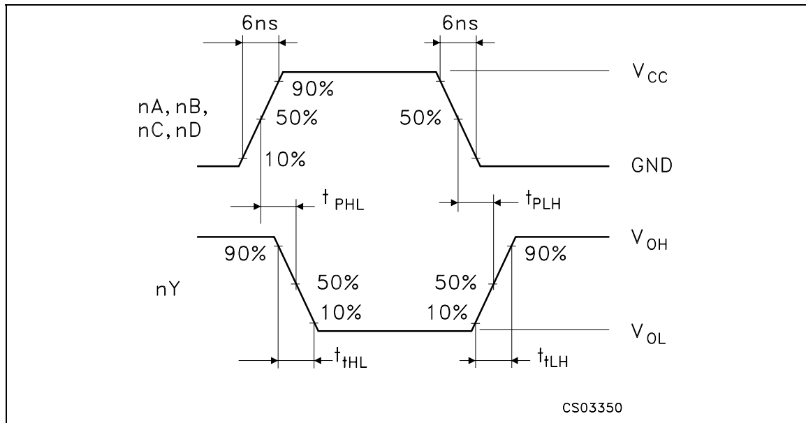
WAVEFORM 1: PROPAGATION DELAY TIME (f=1MHz; 50% duty cycle)
