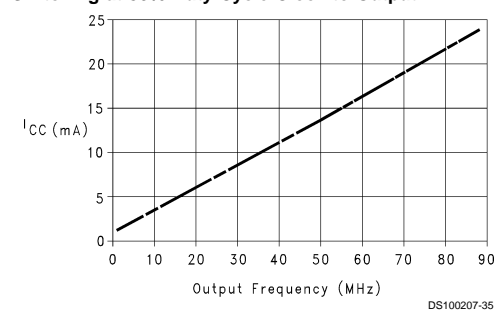
Typical I_{CC} vs Output Switching Frequency C_L = 0 pF, V_{CC} = V_{IH} = 5.5\text{V} , 1 Output Switching at 50% Duty Cycle Clock to Output
