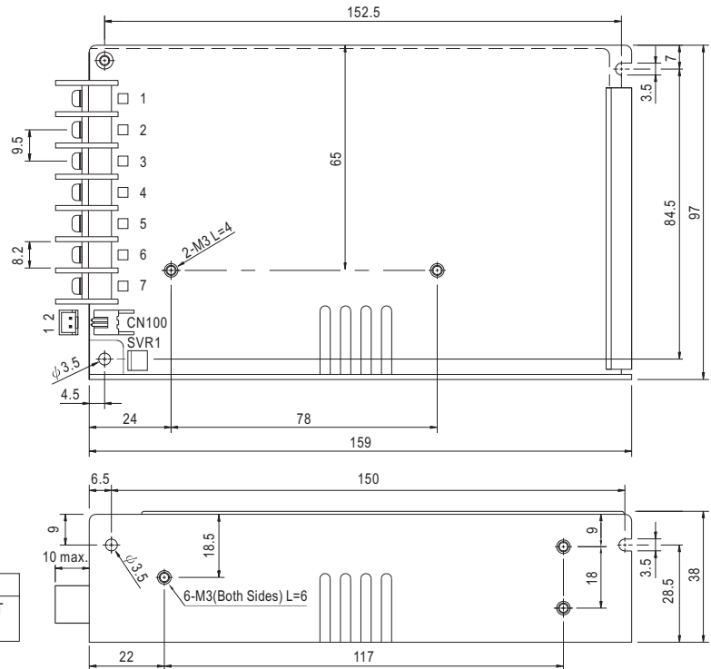
Remote ON/OFF (CN100) : JST B-XH or equivalent
