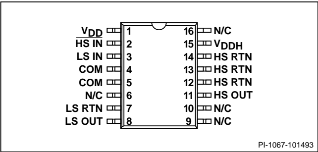
Figure 2. Pin Configuration.
