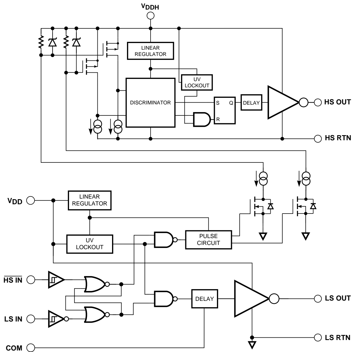
Figure 3. Functional Block Diagram of the INT100
