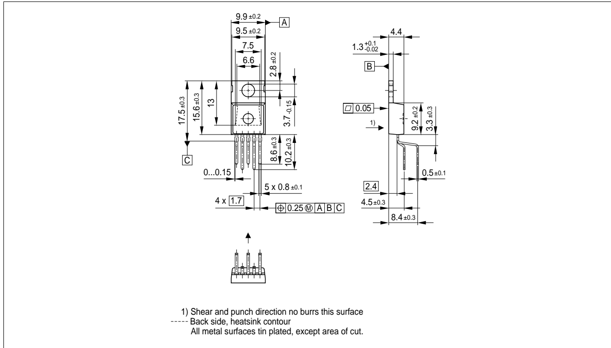
Figure 1 PG-TO220-5-3
