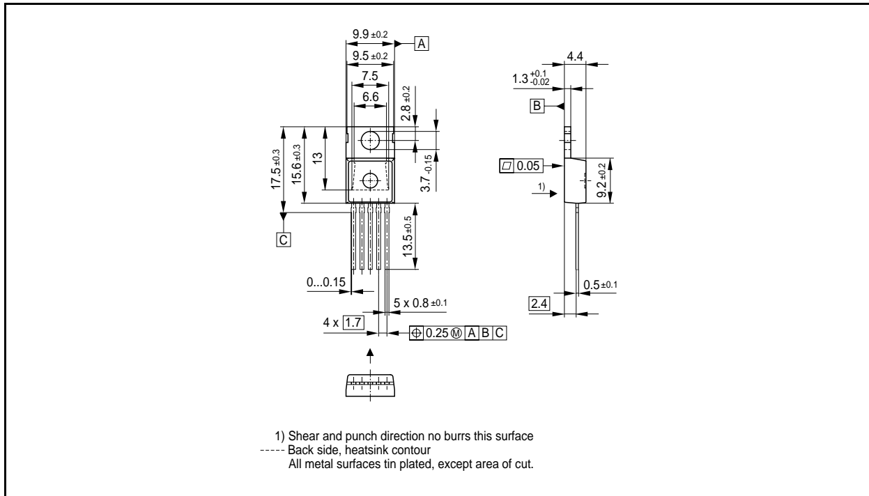
Figure 3 PG-TO220-5-43
