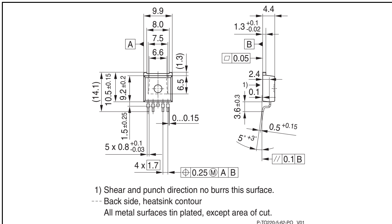
Figure 2 PG-TO220-5-62
