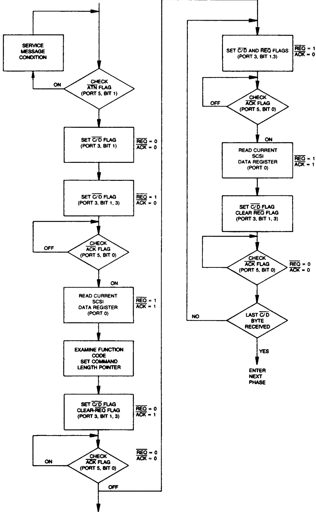
Figure 23. Command Transfer Phase (Target)
