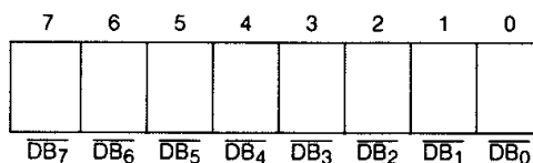
Figure 3. Input Data Register
