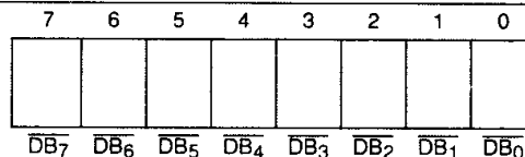
Figure 2. Output Data Register
