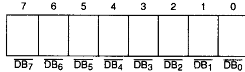
Figure 8. Select Enable Register
