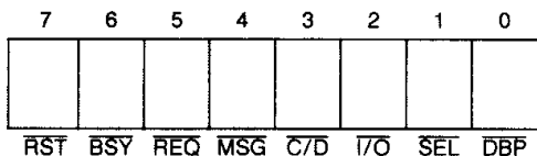
Figure 7. Current SCSI Bus Status Register
