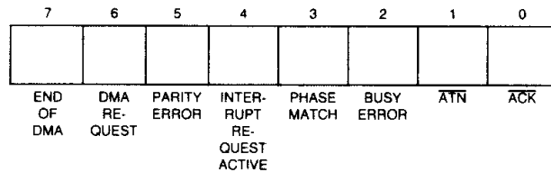
Figure 9. Bus and Status Register
