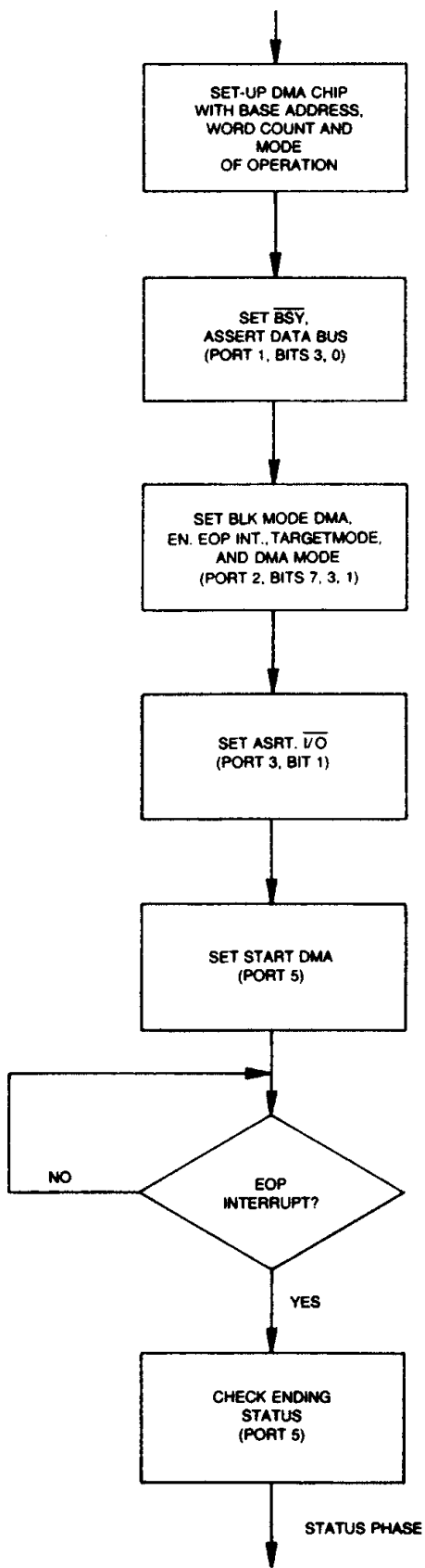
Figure 25. Data Transfer via DMA
