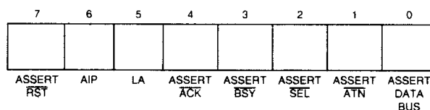
Figure 4-1. Initiator Command Register — Register Read
