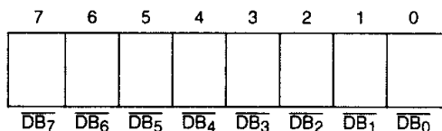
Figure 1. Current SCSI Data Register
