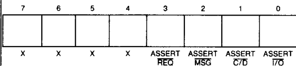
Figure 6. Target Command Register
