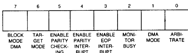
Figure 5. Mode Register
