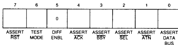
Figure 4-2. Initiator Command Register — Register Write
