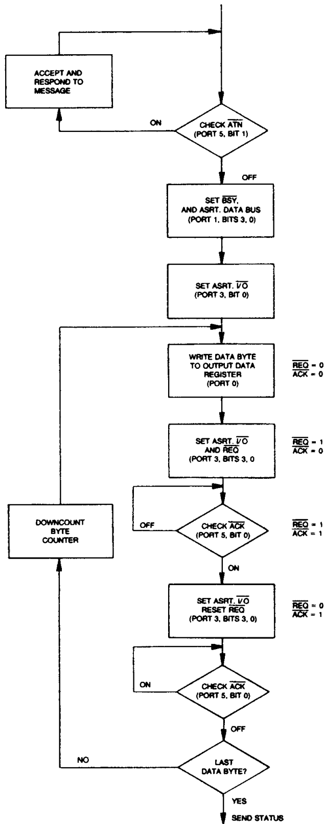
Figure 24. Data Transfer to Host via Programmed I/O
