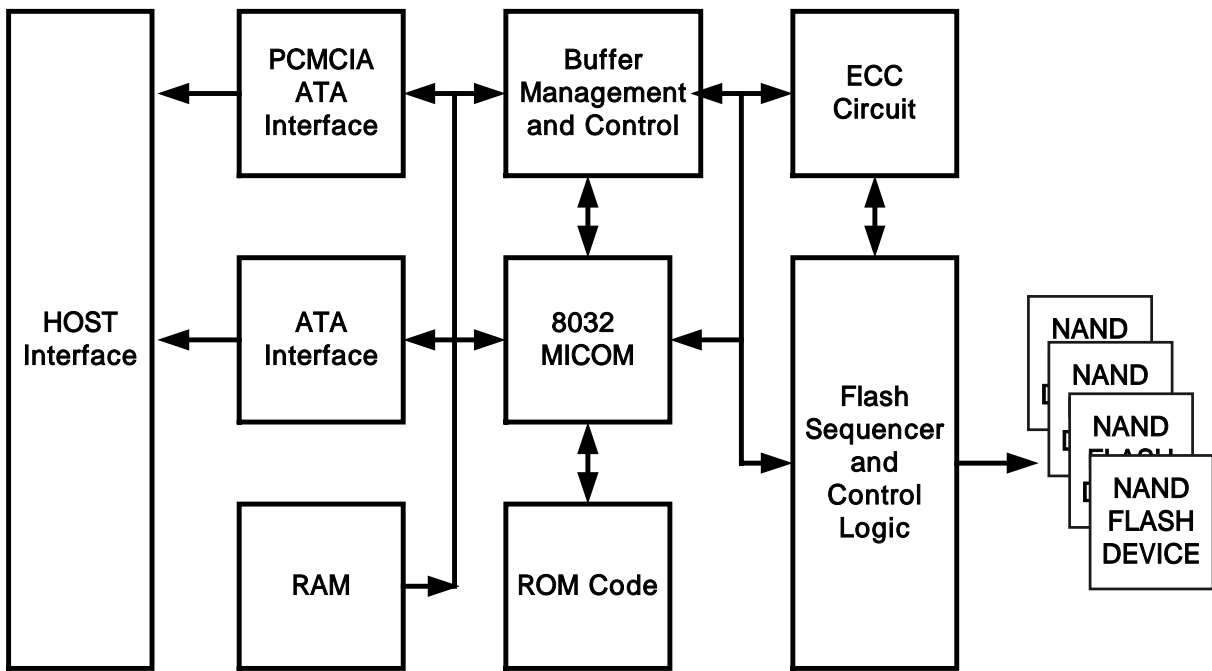
Figure 2.1 Block Diagram
