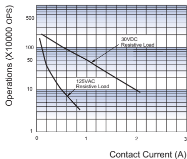
ENDURANCE CURVE
