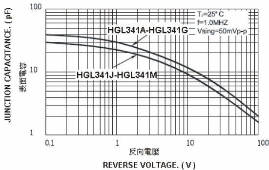
FIG. 5 – 表面電容(典型值) FIG. 5 – TYPICAL JUNCTION CAPACITANCE
