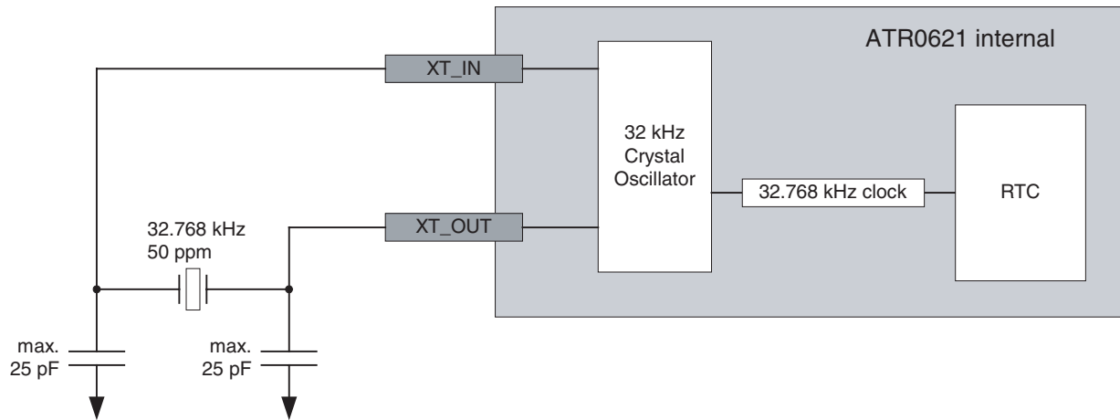
Figure 4-1. Crystal Connection
