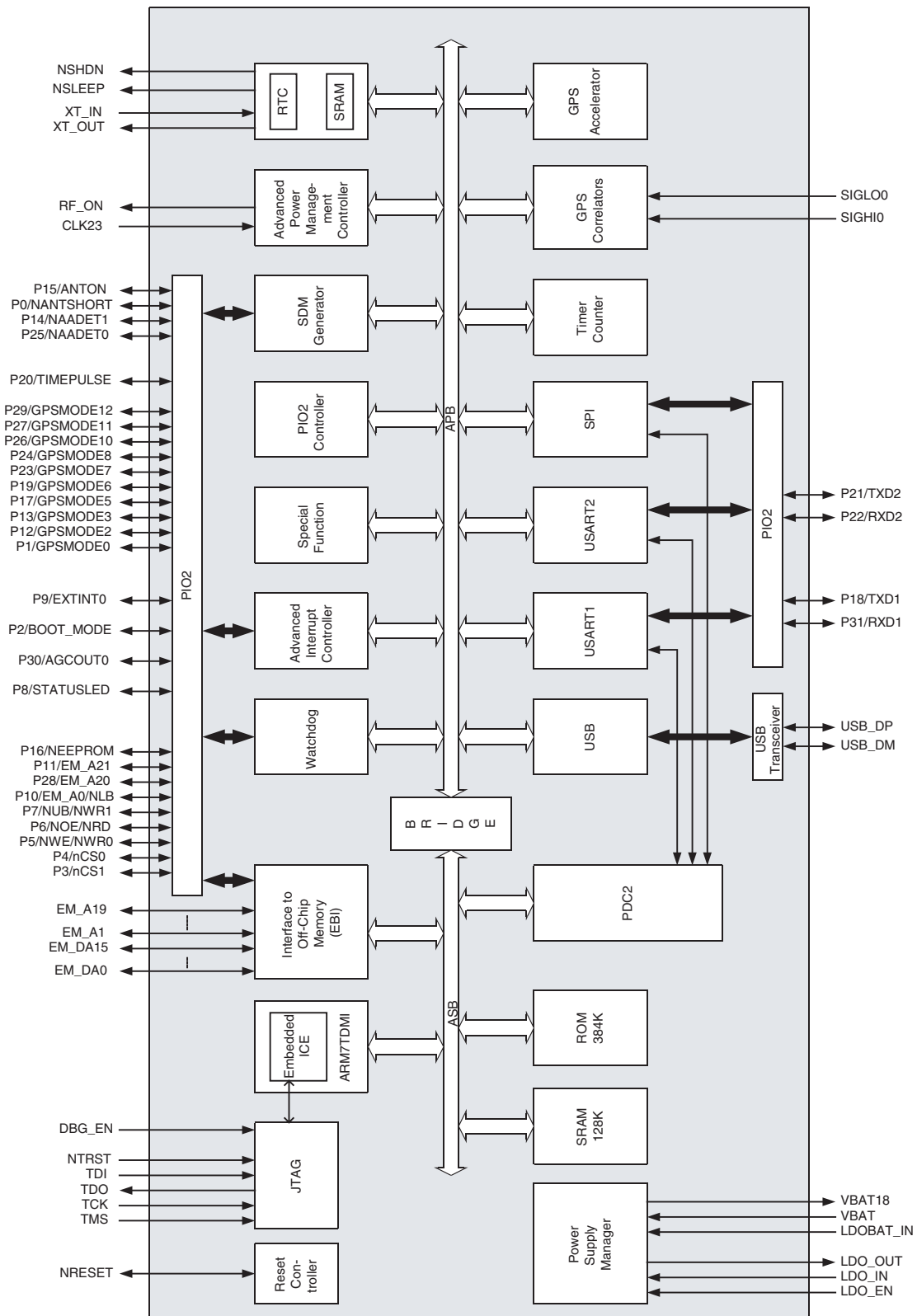
Figure 1-1. Block Diagram
