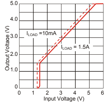
Figure 3. GM66150-5.0 Dropout Characteristics
