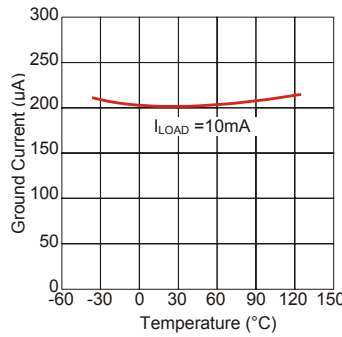
Figure 5. GM66150 Ground Current vs. Temperature
