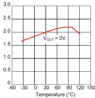
Figure 8. GM66150-3.3 Short Circuit Current vs. Temperature
