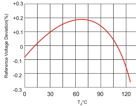
Figure 4. Bandgap Reference Voltage Deviation vs. Temperature
