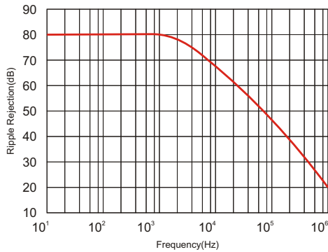
Figure 5. Ripple Rejection vs. Frequency
