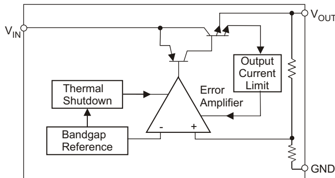
(Fixed Version)
