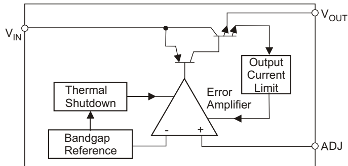
(Adjustable Version)
