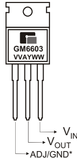
TO-220
