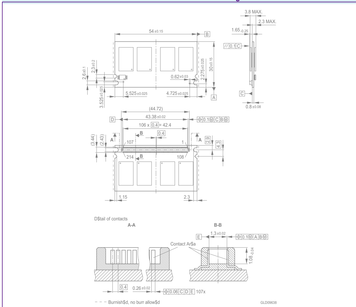
FIGURE 5 Package Outline Raw Card A L-DIM-214-1
