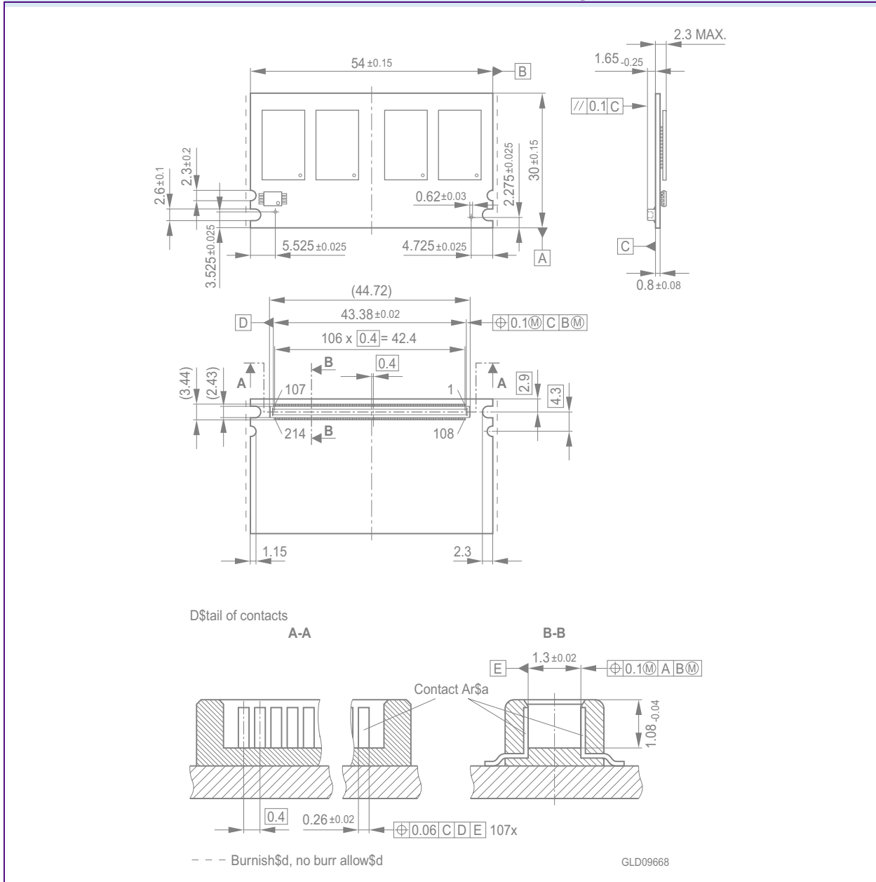
FIGURE 6 Package Outline Raw Card B L-DIM-214-2
