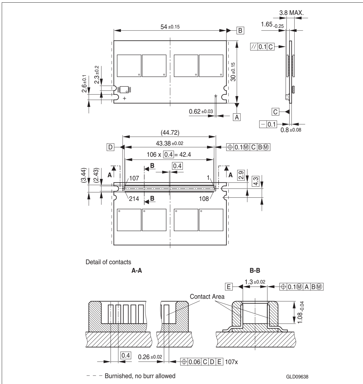
Figure 4 PCB Raw Card A Component Placement L-DIM-214-1
