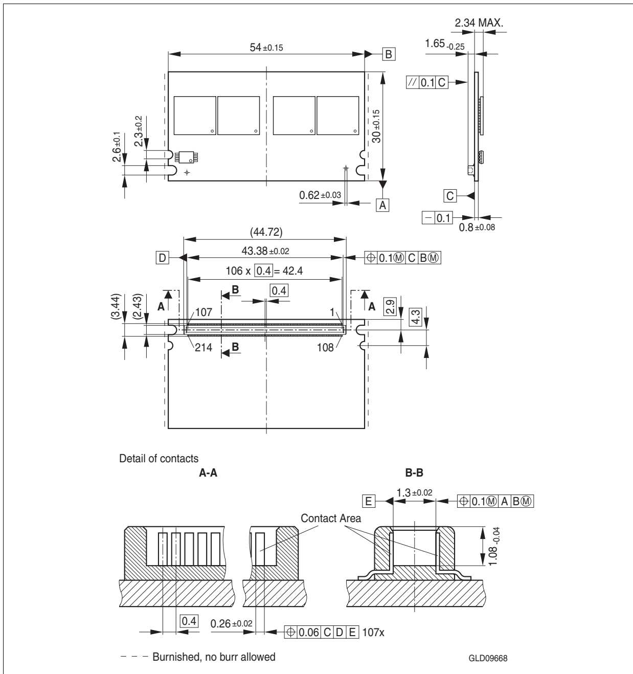
Figure 5 PCB Raw Card B Component Placement L-DIM-214-2
