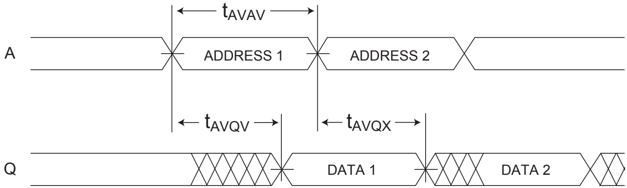
FIG. 2 TIMING WAVEFRONT - READ CYCLE
