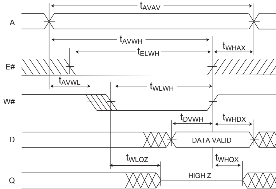
FIG. 3 WRITE CYCLE - W# CONTROLLED
