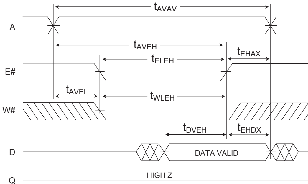
FIG. 4 WRITE CYCLE - E# CONTROLLED
