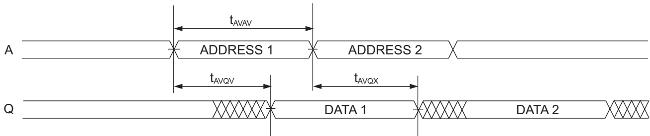
FIG. 4 READ CYCLE 1 - W# HIGH, G#, E# LOW
