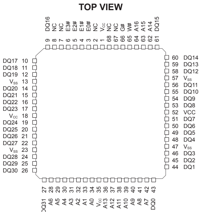
FIG. 1 PIN CONFIGURATION
