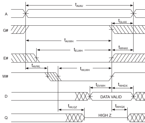
FIG. 6 WRITE CYCLE 1 - W# CONTROLLED
