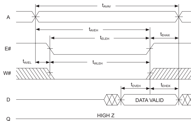
FIG. 7 WRITE CYCLE 2 - E# CONTROLLED
