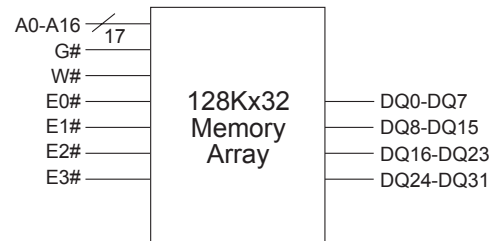
BLOCK DIAGRAM
