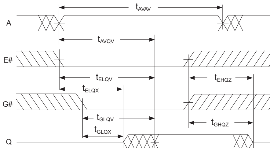
FIG. 5 READ CYCLE 2 - W# HIGH
