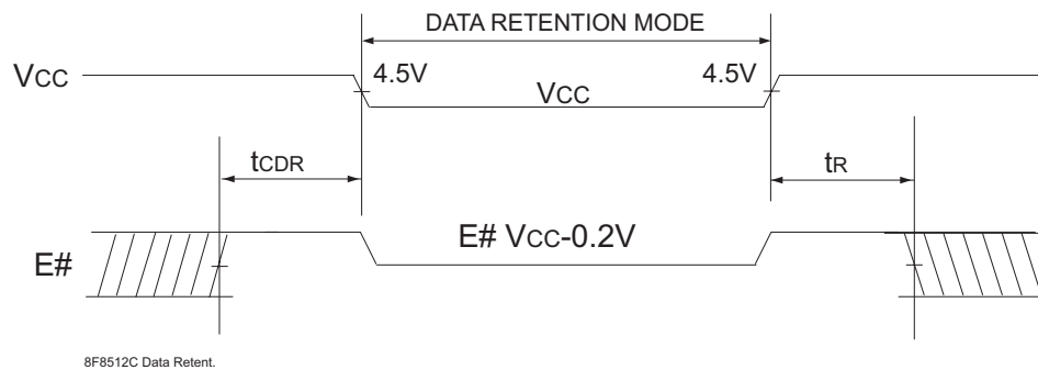
FIG. 9 DATA RETENTION E# CONTROLLED
