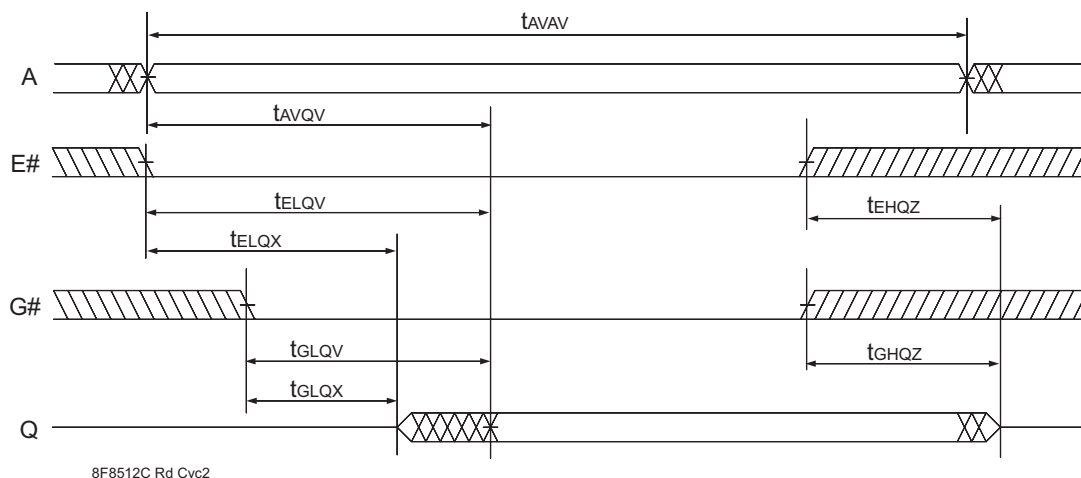
FIG. 4 READ CYCLE 2 - W# HIGH
