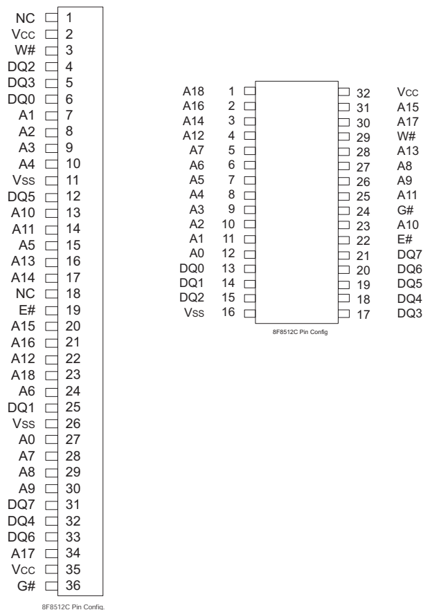
FIG. 1 PIN CONFIGURATIONS
