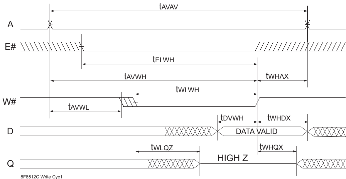
FIG. 7 WRITE CYCLE 1 - W# CONTROLLED
