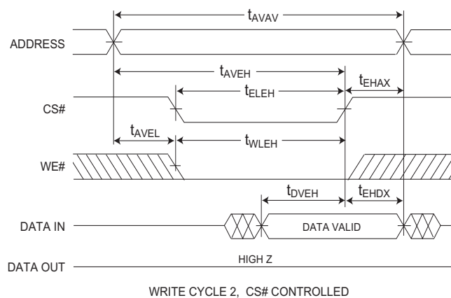
FIG. 4 WRITE CYCLE - CS# CONTROLLED
