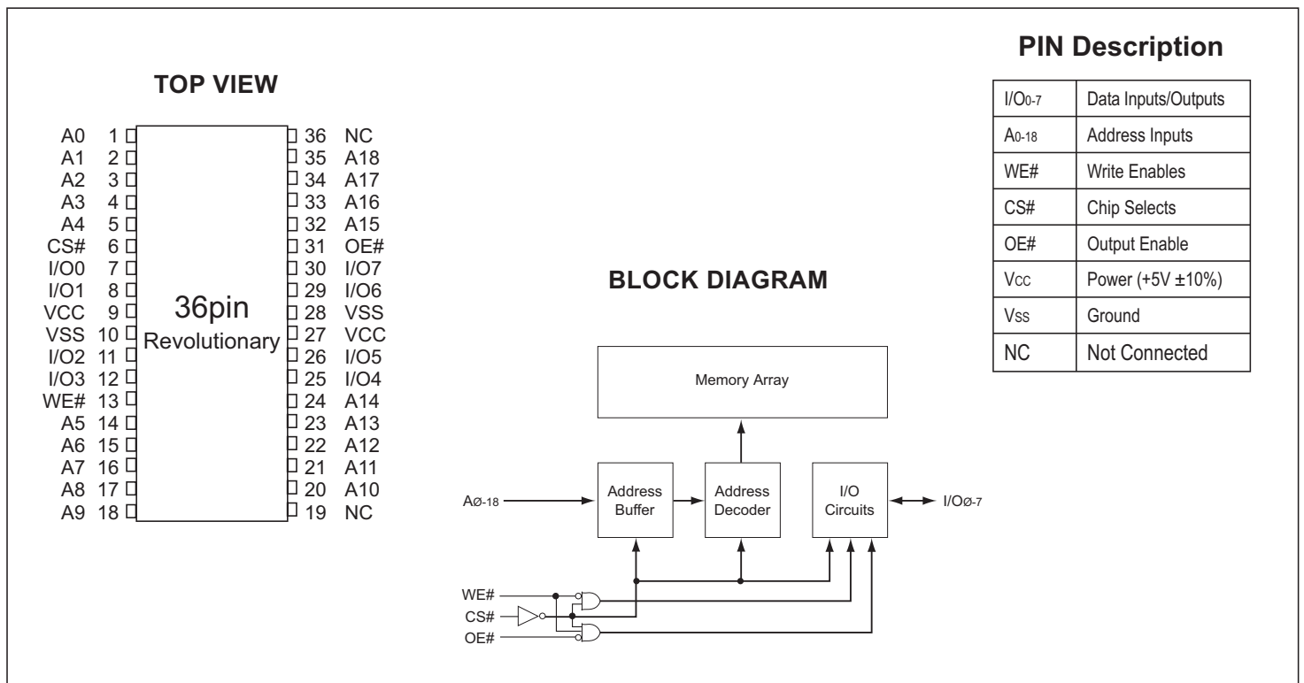
FIG. 1 – PIN CONFIGURATION
