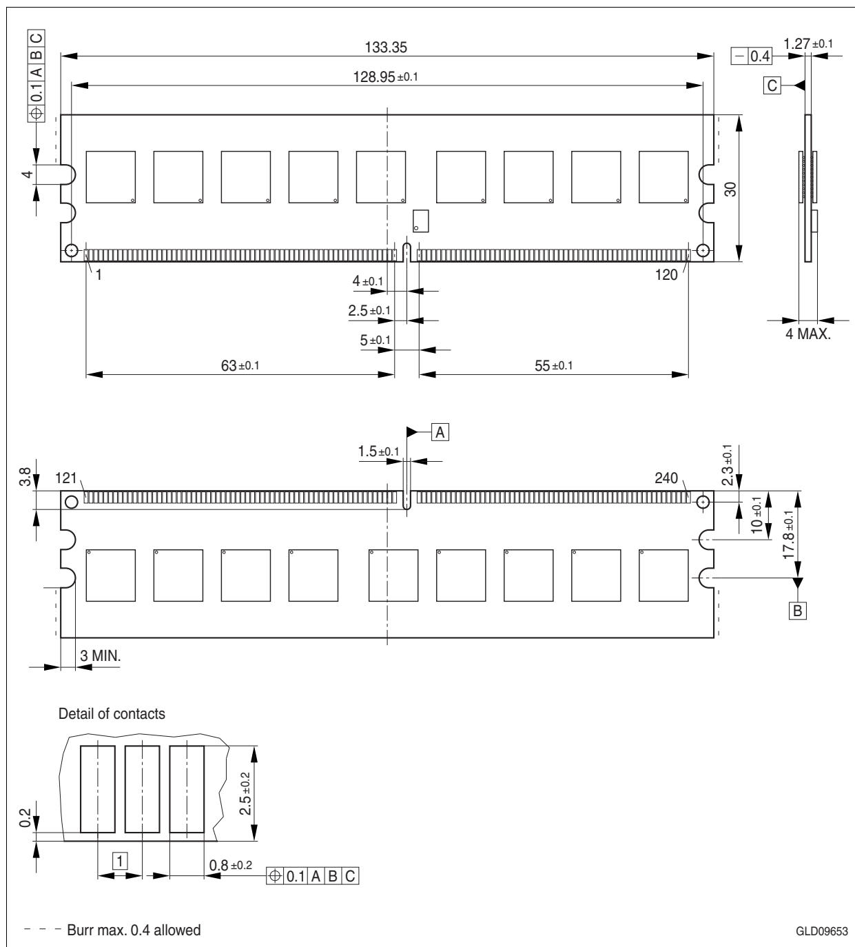
Figure 9 Package Outline L-DIM-240-2
