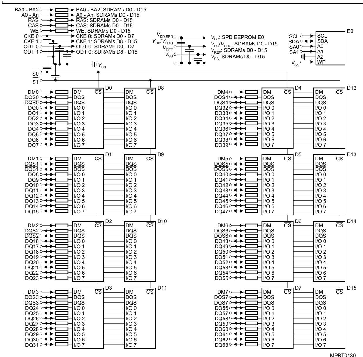
Figure 5 Block Diagram Raw Card B UDIMM (x64, 1 Rank, x8)
