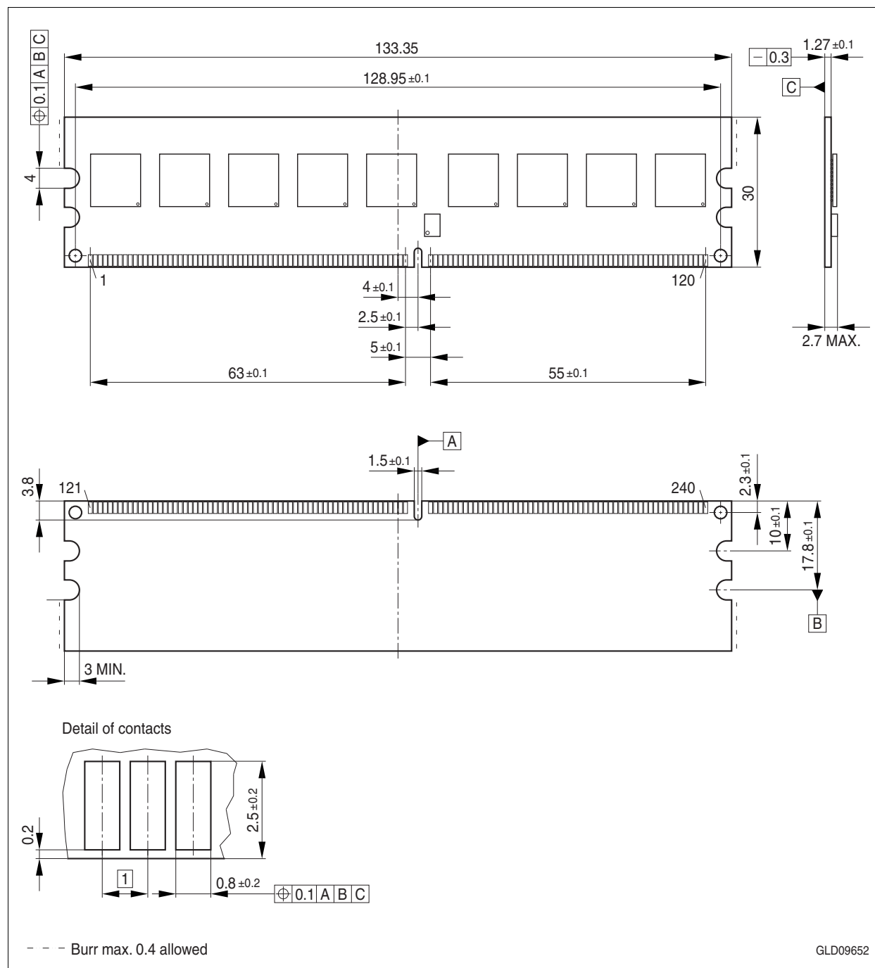
Figure 8 Package Outline L-DIM-240-1
