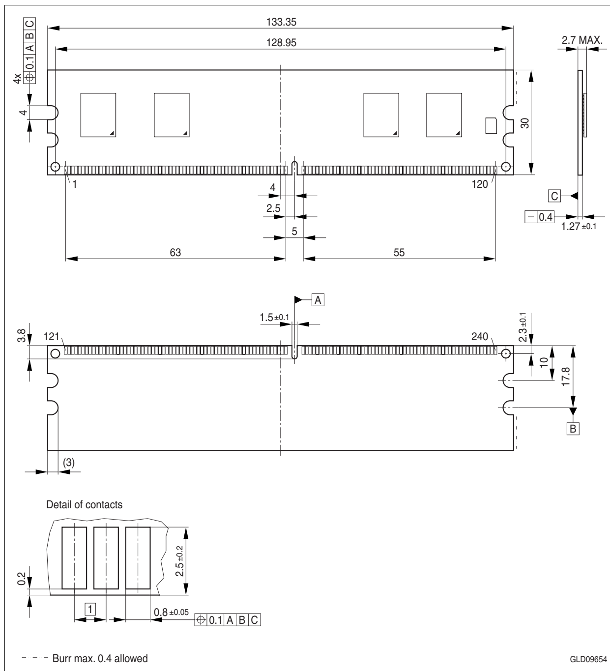
Figure 10 Package Outline L-DIM-240-3
