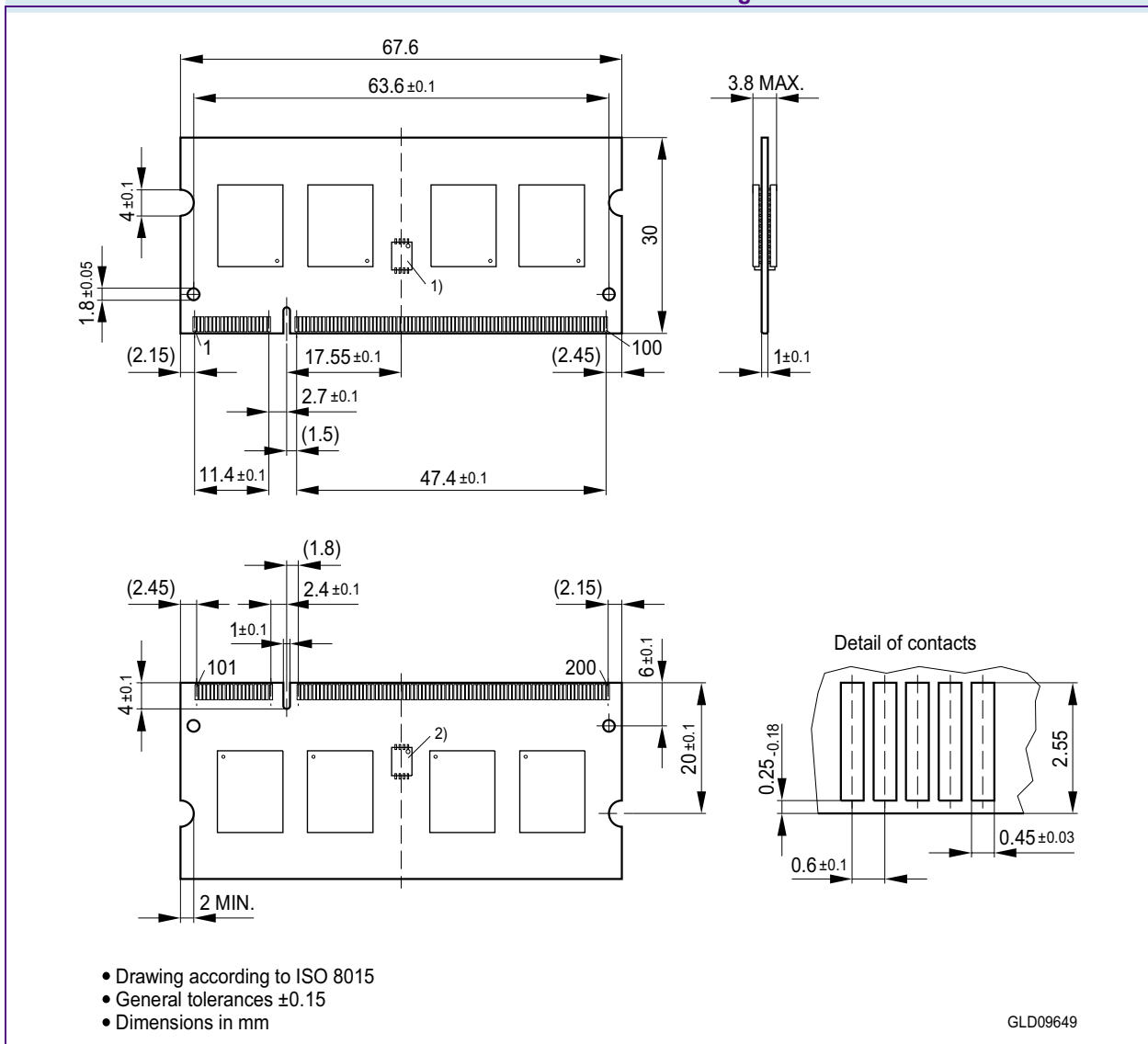
FIGURE 5 Package Outline Raw Card A L-DIM-200-31
