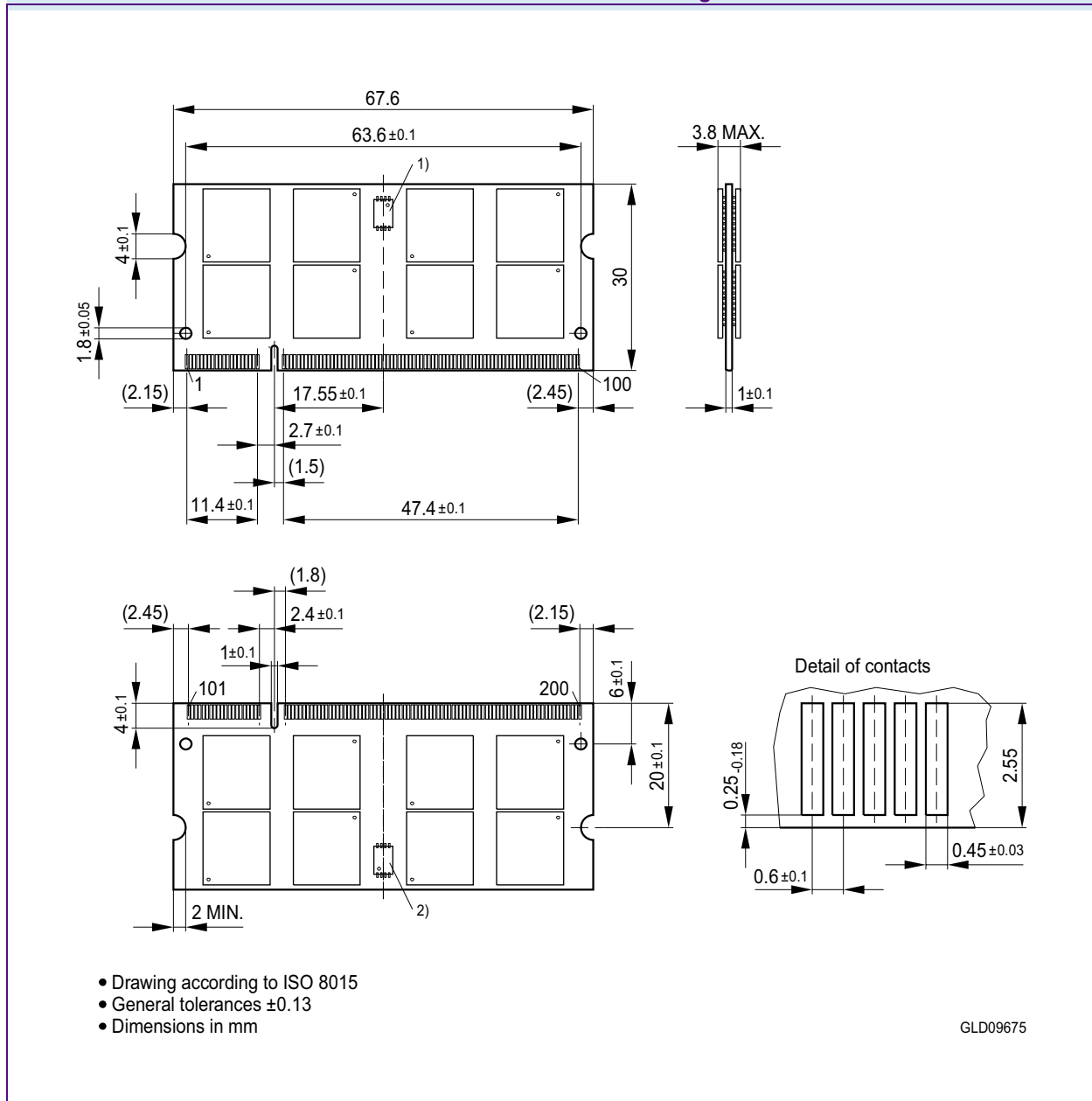
Package Outline Raw Card F - L-DIM-200-34
