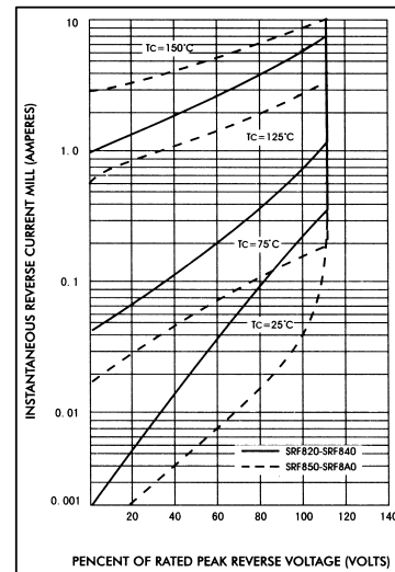
FIG.3-TYPICAL REVERSE CHARACTERISTICS
