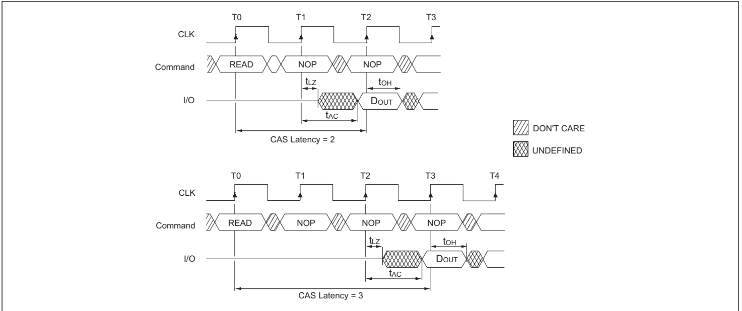
FIGURE 4 – CAS LATENCY
