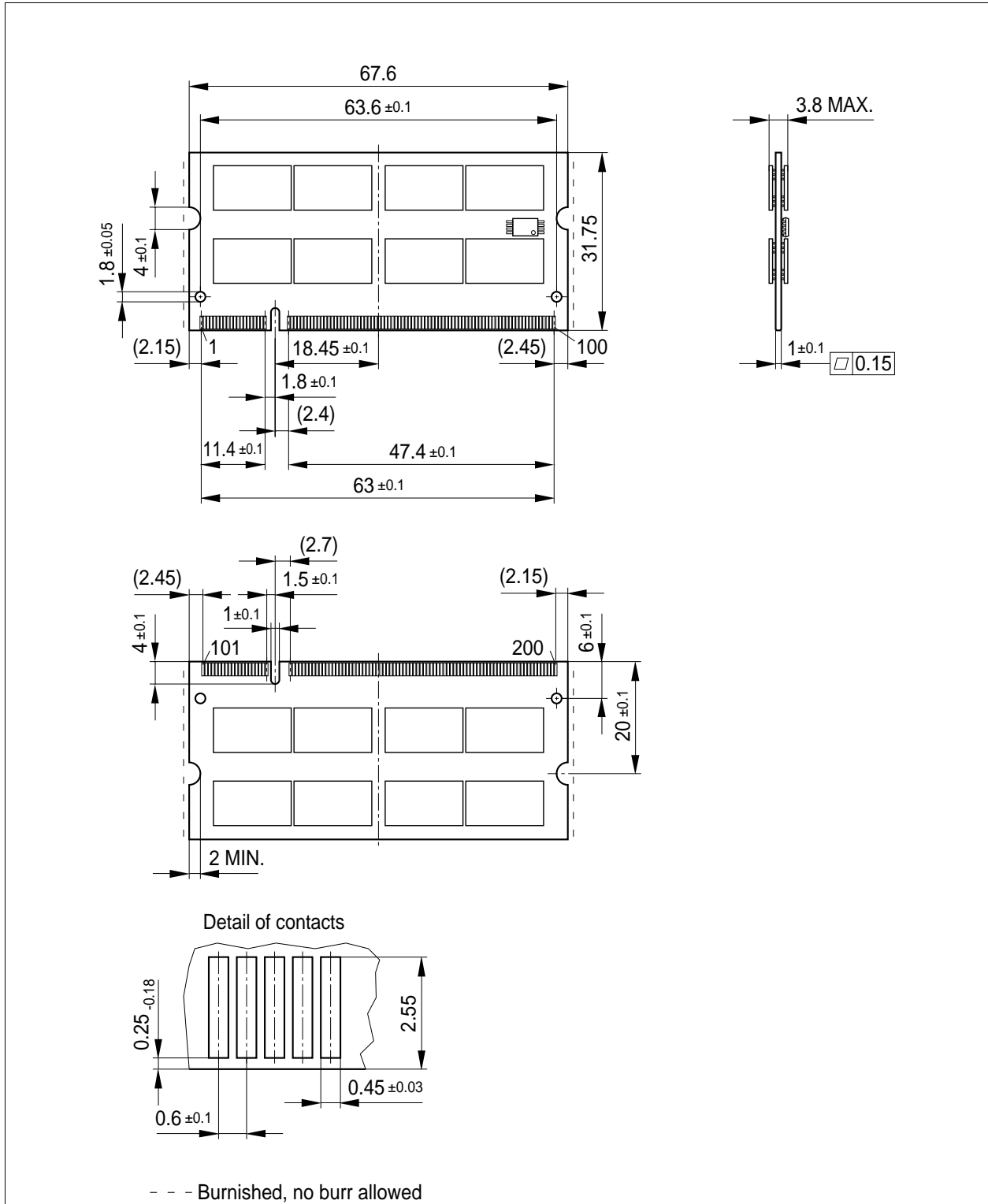
Figure 3 Package Outline SO-DIMM Raw Card Z (L-DIM-200-9)
