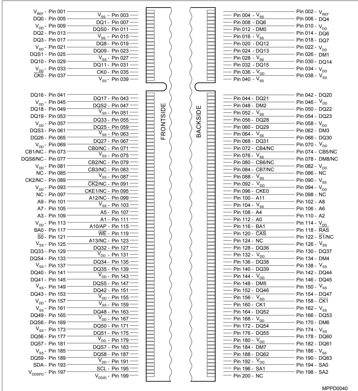
Figure 1 Pin Configuration Diagram 200-Pin SO-DIMM
