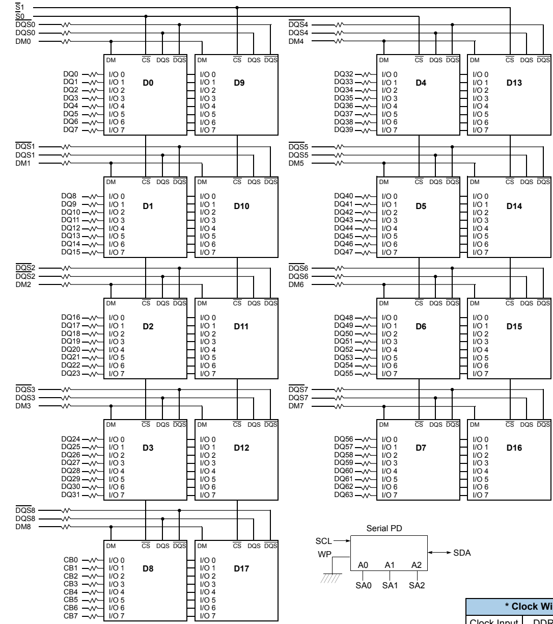
Functional Block Diagram: 1GB, 128Mx72 ECC Module (Populated as 2 ranks of x8 DDR2 SDRAMs) M391T2953BG(Z)3 / M391T2953BG(Z)0
