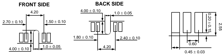
DETAIL a
