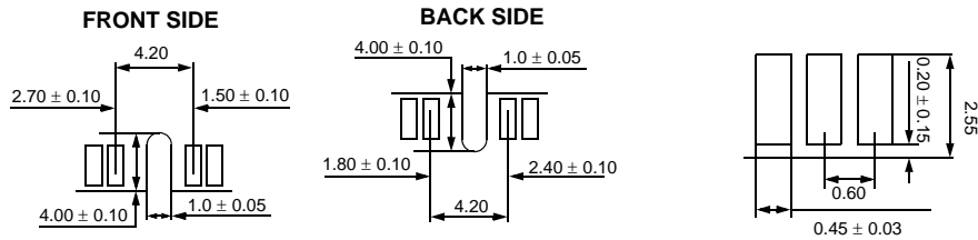
DETAIL a
