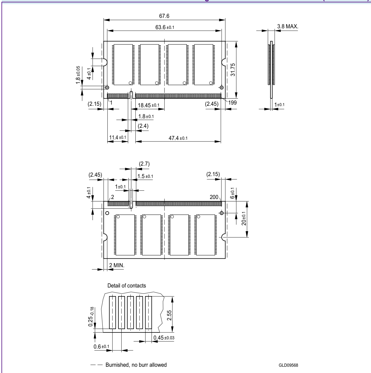
FIGURE 4 Package Outline SO-DIMM Raw Card A (L-DIM-200-6)
