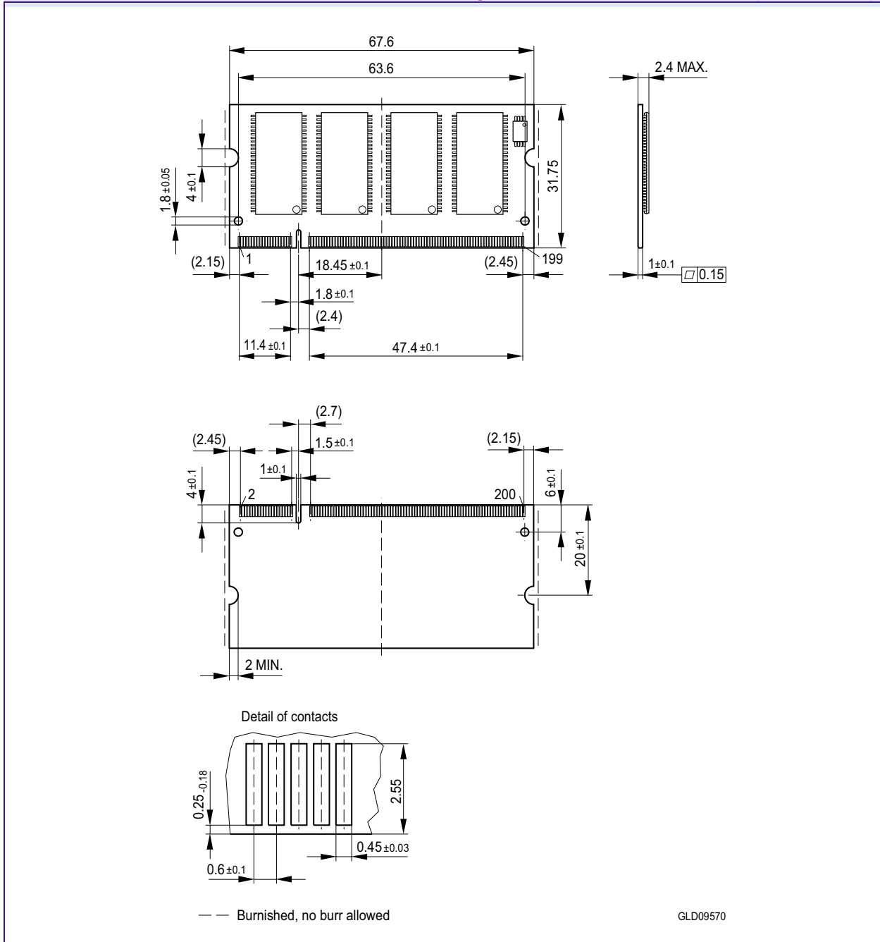
Package Outline SO-DIMM Raw Card C (L-DIM-200-11)
