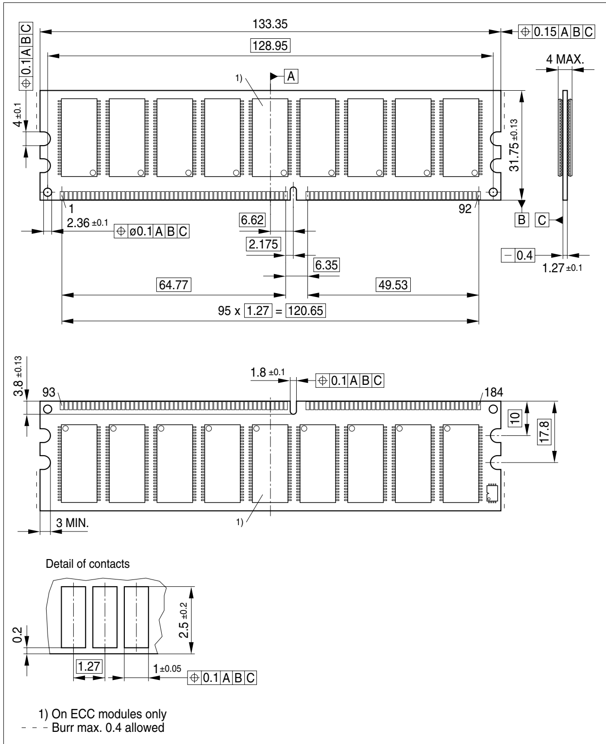
Figure 6 DDR-SDRAM DIMM Module Package
