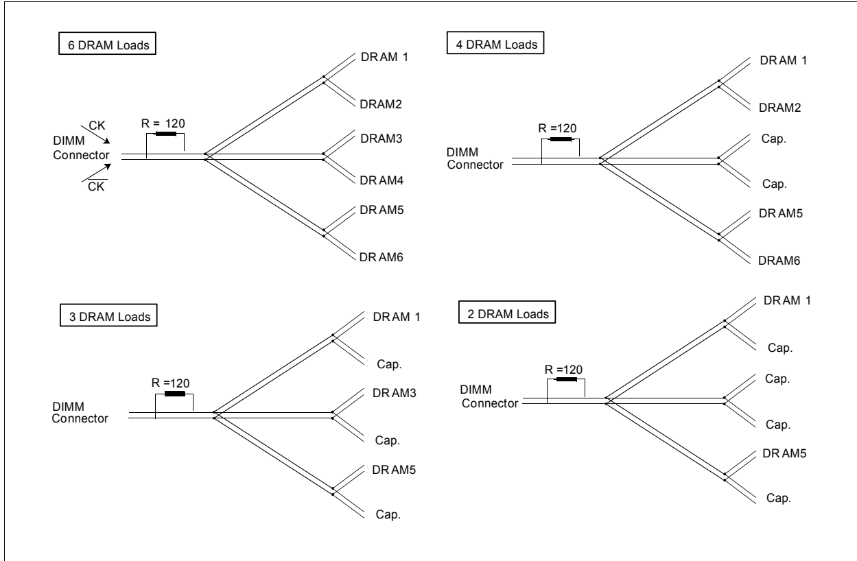
Figure 5 Clock Net Wiring
