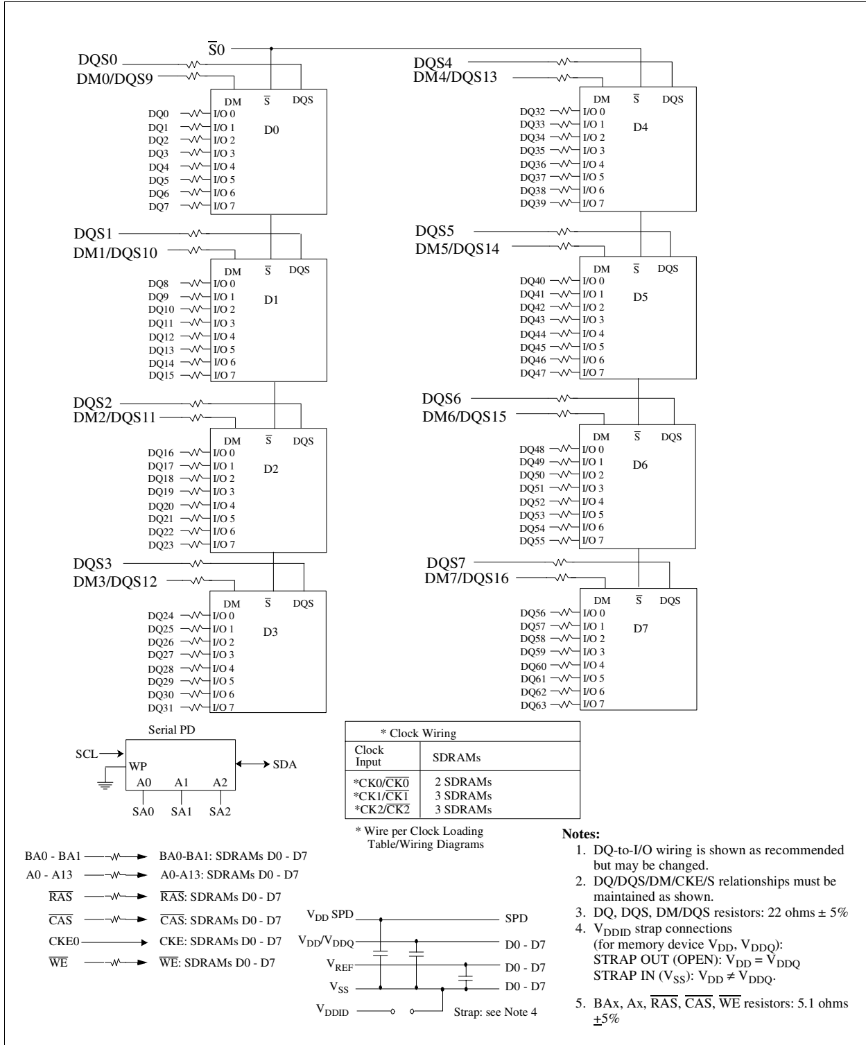
Figure 1 Block Diagram: One Rank 16M x 64 DDR SDRAM DIMM Module HYS64D16000GU using x8 organized SDRAMs
