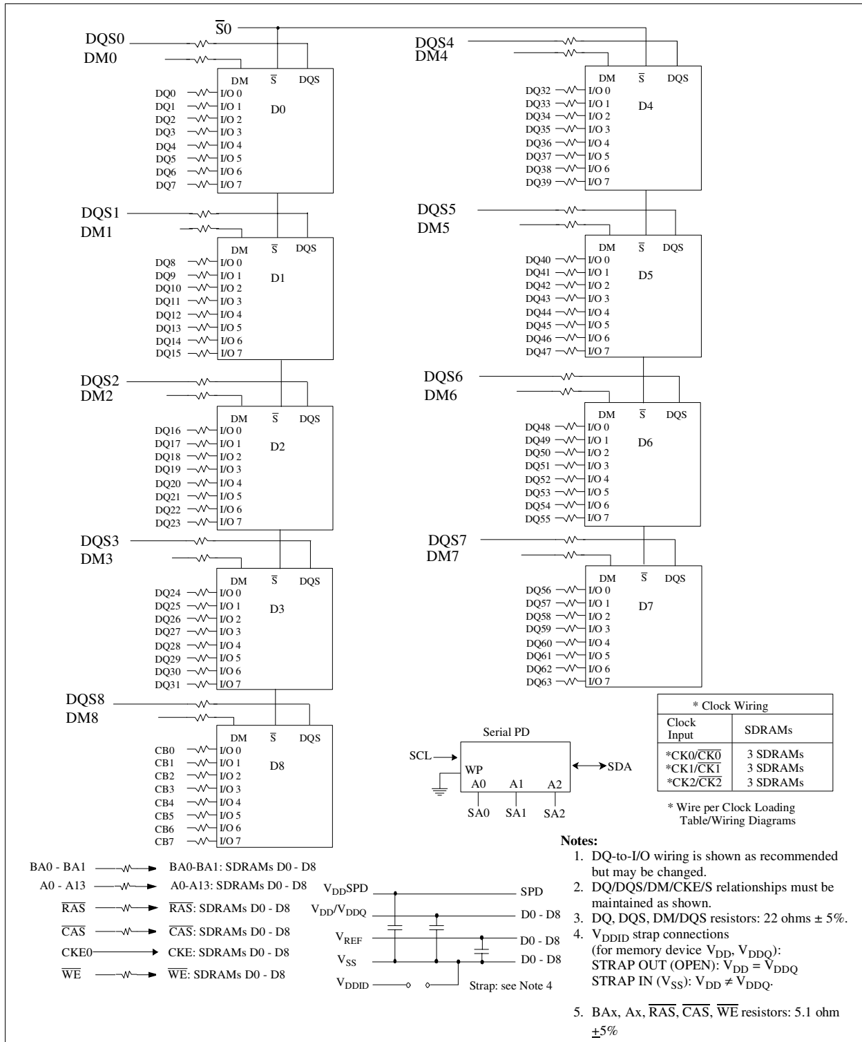
Figure 3 Block Diagram: One Rank 16M \times 72 DDR SDRAM DIMM Module HYS72D16000GU using \times 8 organized SDRAMs
