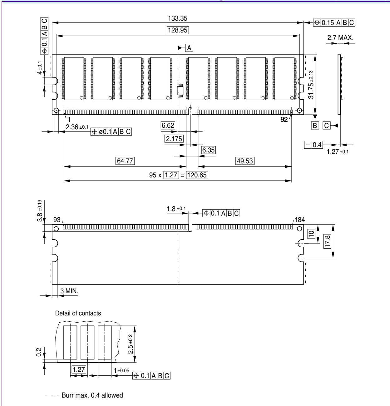
Package Outline UDIMM Raw Card A (L-DIM-184-32)
