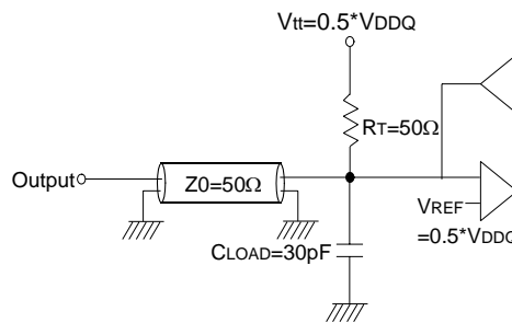
Output Load Circuit (SSTL_2)
