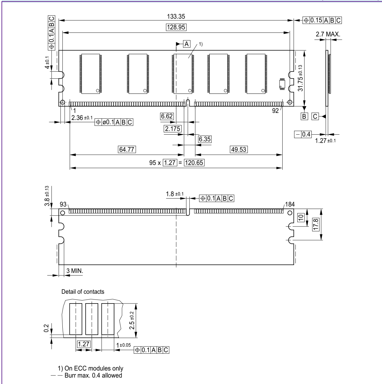
Raw Card C DDR UDIMM HYS64D32301HU-5-B (1 Rank Module)
