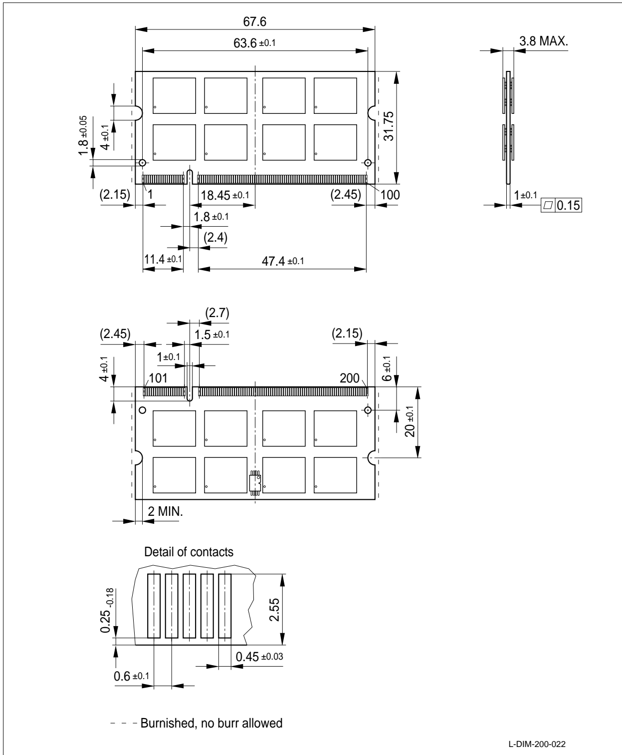
Figure 3 Package Outlines – DDR-SDRAM SO-DIMM HYS64D128021[H/G]BDL-[5/6]-B
