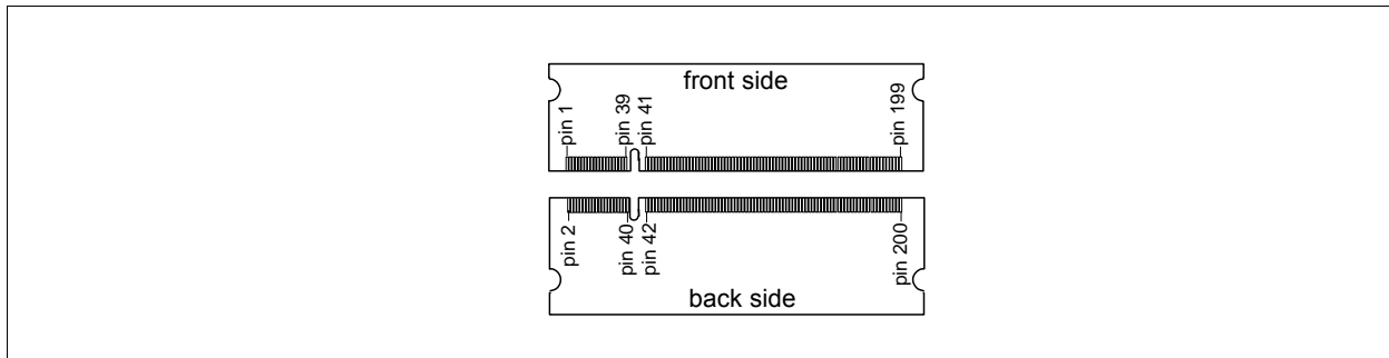
Figure 1 Pin Configuration
