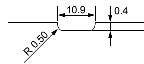
Detail C
