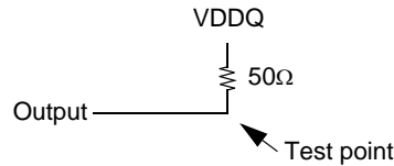
Figure 3 : Pulldown slew rate test load
