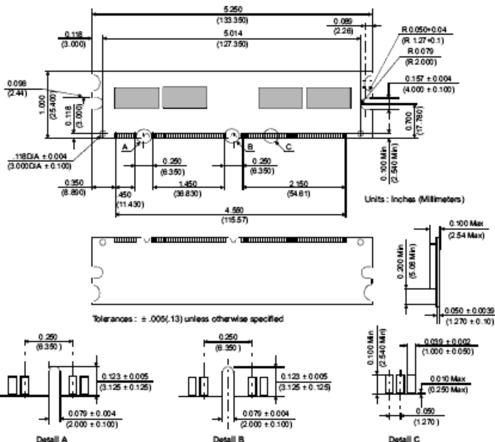
Figure 1: KVR133X64C3L/128 168-Pin SDRAM Module
