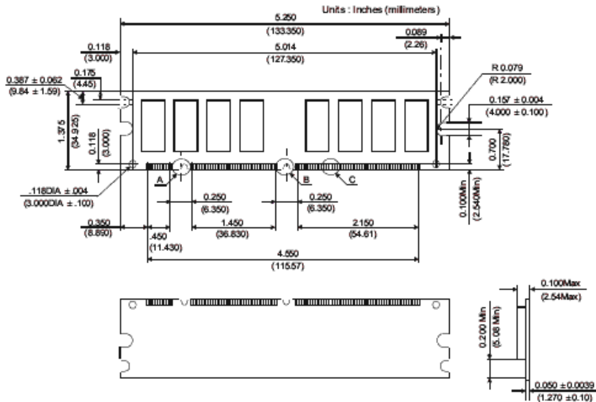
Figure 1: KVR133X64C3/64 168-Pin SDRAM Module
