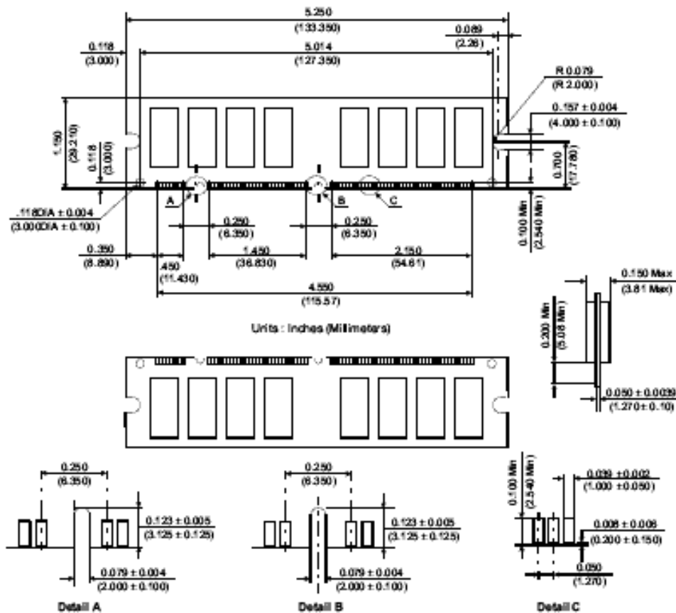
Figure 1: KVR133X64C3/1G 168-Pin SDRAM Module
