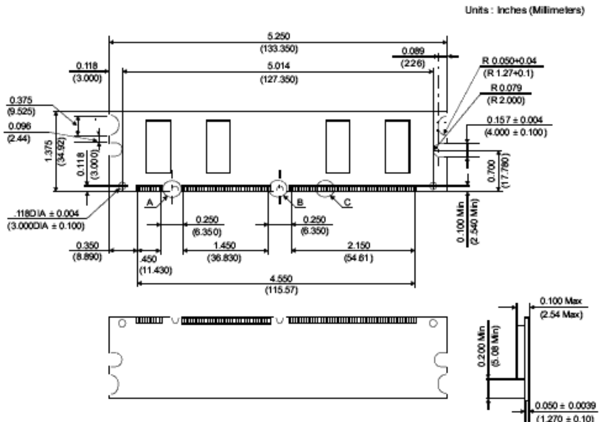
Figure 1: KVR133X64C3/128 168-Pin SDRAM Module
