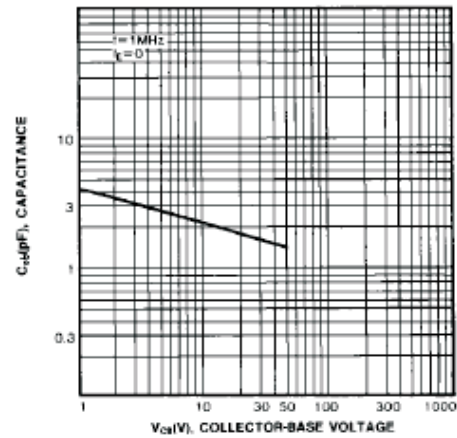
Fig.6 Output Capacitance
