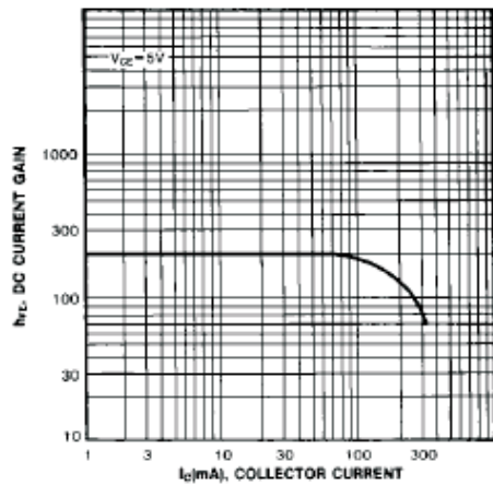
Fig.3 DC Current Gain
