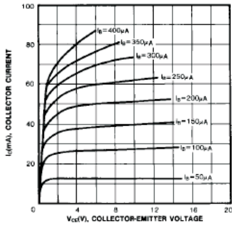
Fig.1 Static Characteristic
