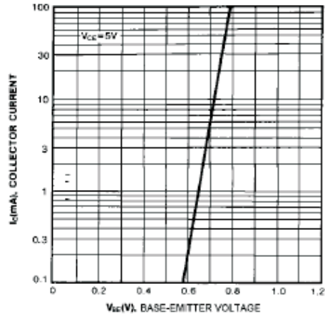
Fig.2 Transfer Characteristic
