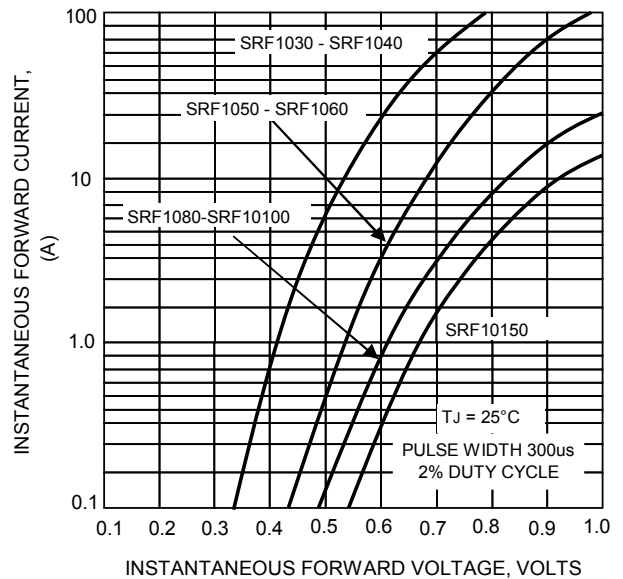
FIG.4-TYPICAL FORWARD CHARACTERISTICS
