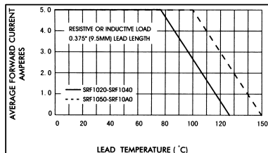
FIG.1-FORWARD CURRENT DERATING CURVE
