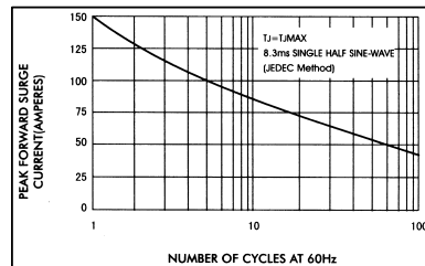
FIG.2-MAXIMUM NON-REPETITIVE PEAK FORWARD SURGE CURRENT
