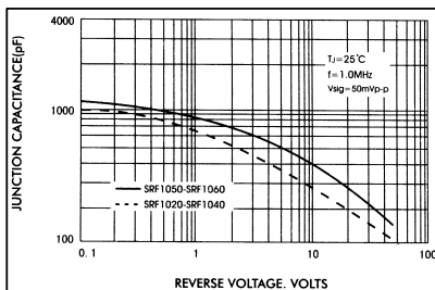
FIG.5-TYPICAL JUNCTION CAPACITANCE
