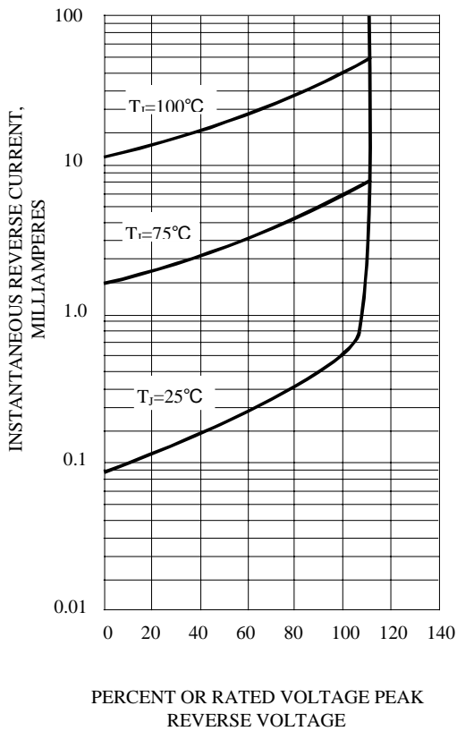
FIG. 3 - TYPICAL REVERSE CHARACTERISTICS
