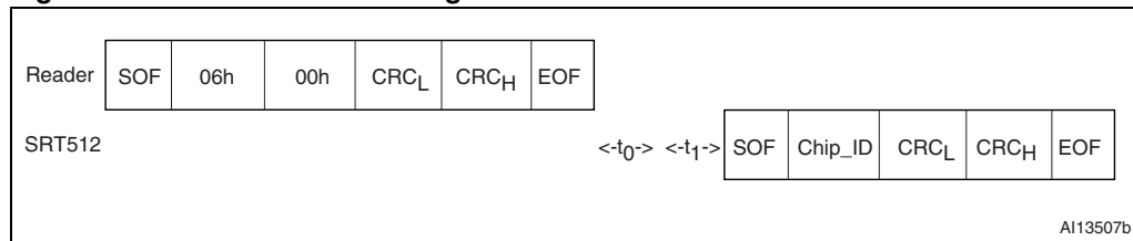
Figure 24. Initiate frame exchange between reader and SRT512
