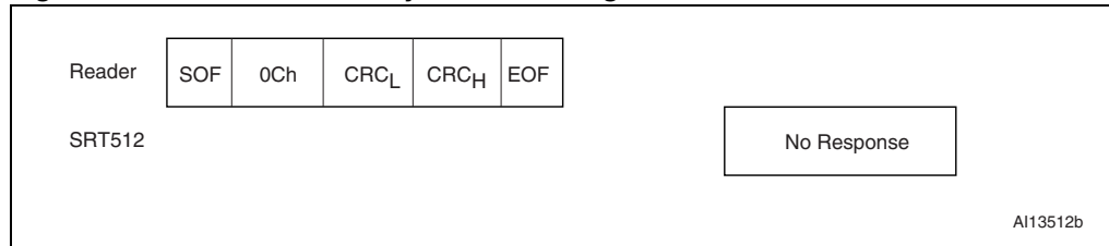
Figure 57. Read_block frame exchange between reader and SRT512
