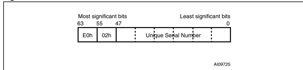
Figure 13. UID format
