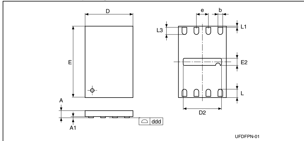
Figure 42. UFDFPN8 (MLP8), 8-lead ultra thin fine pitch dual flat package no lead 2 × 3 mm, package outline
