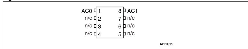
Figure 2. MLP connections
