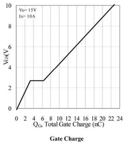
Gate Charge
