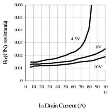
On-Resistance vs. Drain Current
