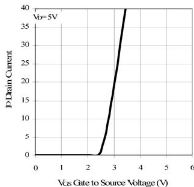
Transfer Characteristics
