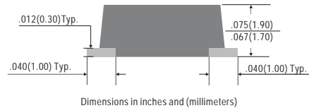
Dimensions in inches and (millimeters)
