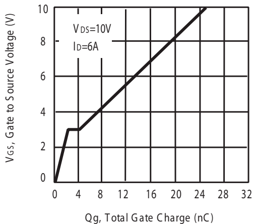
Figure 9. Gate Charge
